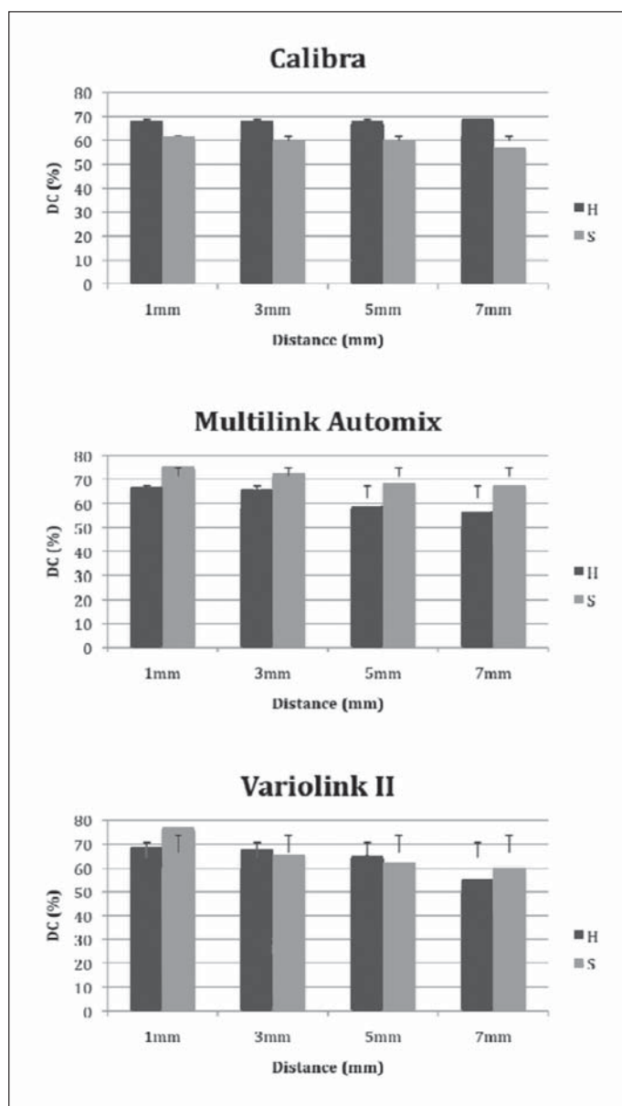
Fig. 2. Percentage degree of conversion reached by the tested materials when cured according to the H (1200 mW/cm 2 for 40 seconds) and the S mode (400 mW/cm 2 for 120 seconds). Increasing the distance from the light tip brings to a drawback in the material performances in all the tested composites except for Calibra.
